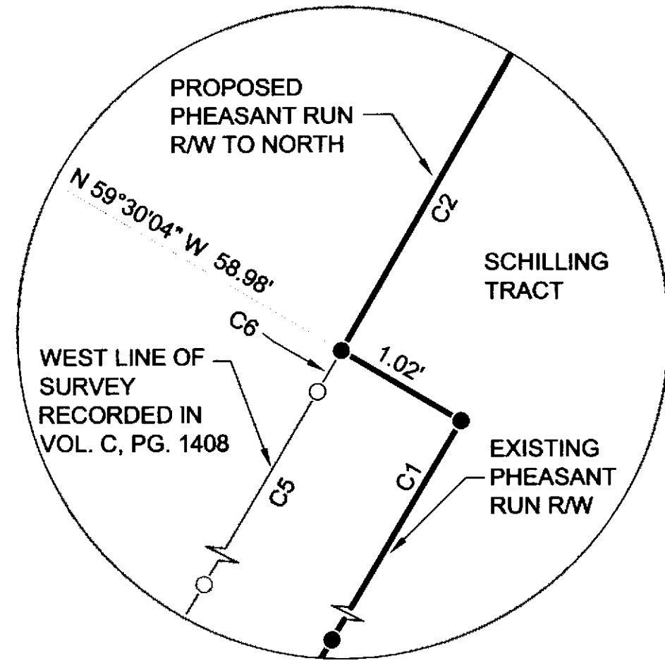
DETAIL B 1" = 1'
