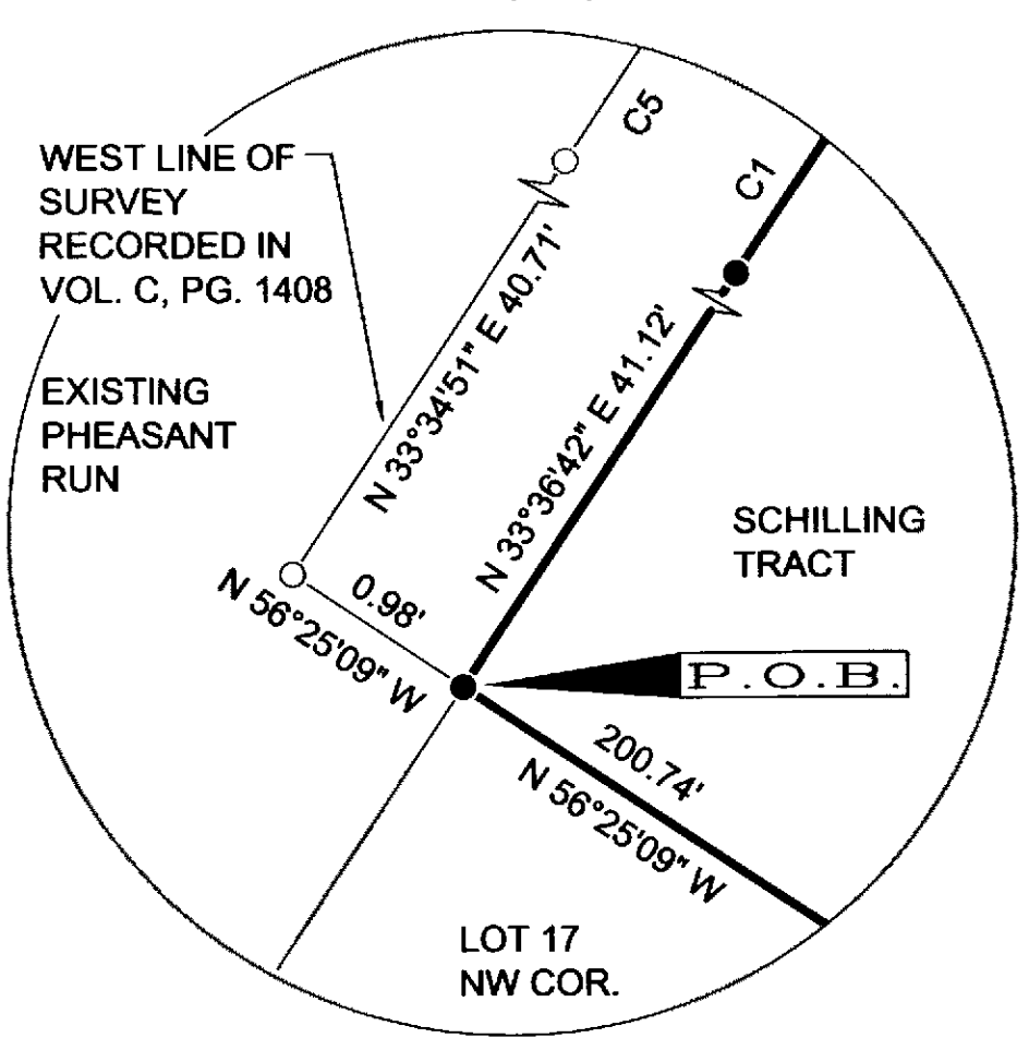
DETAIL A 1" = 1'
