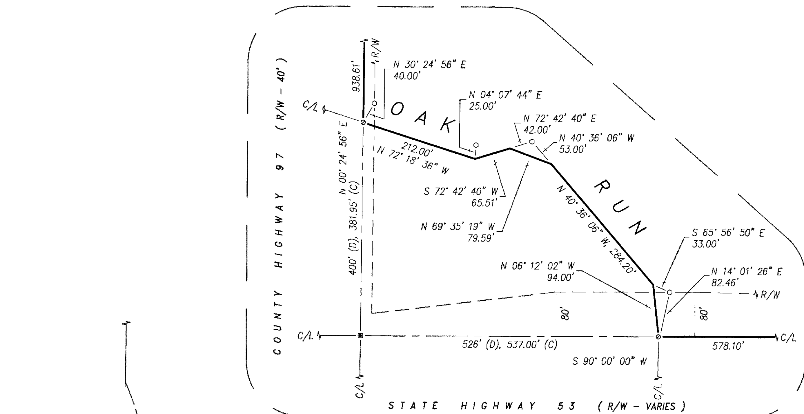
DETAIL A SCALE 1"=100'
