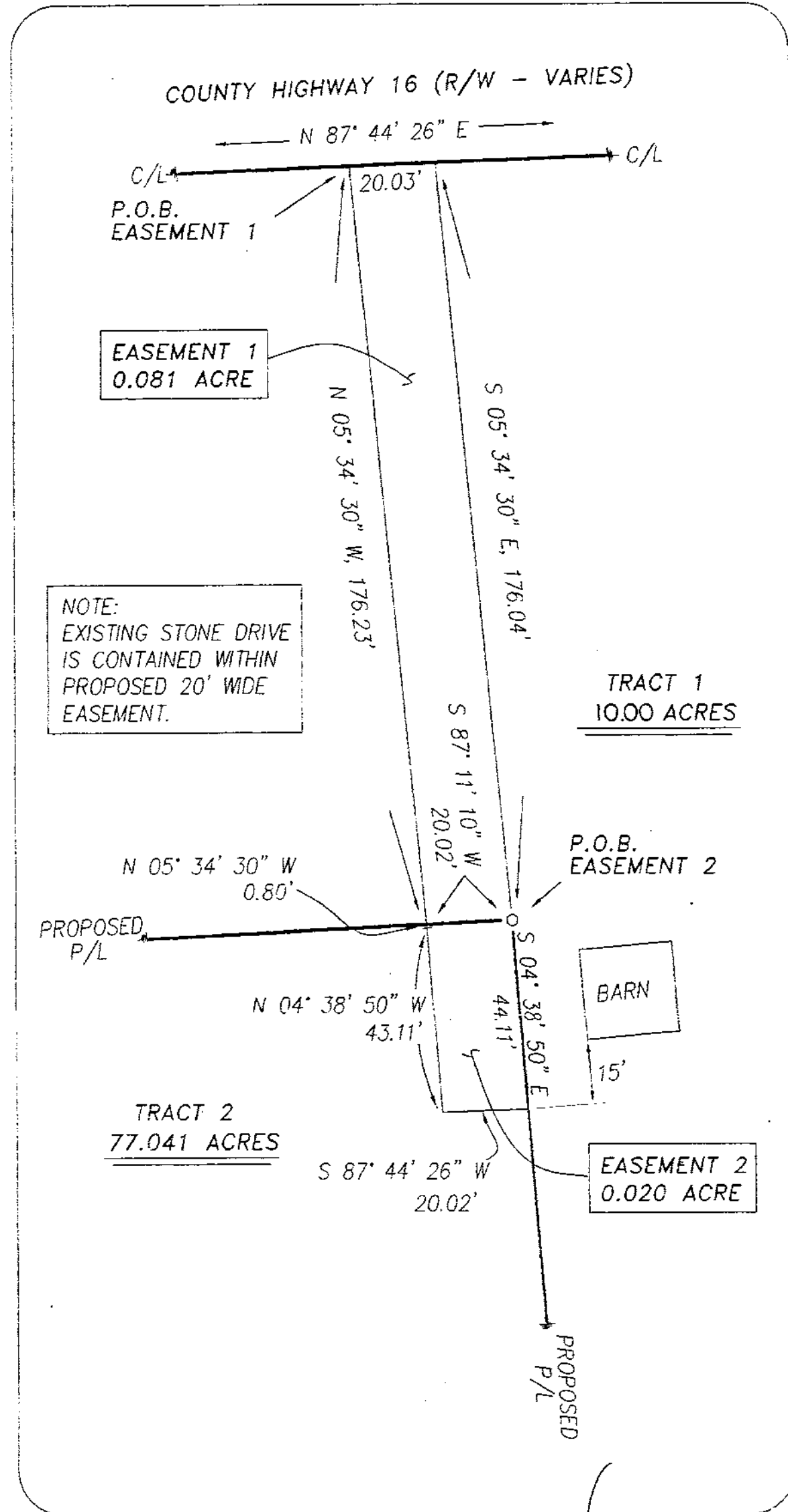
EASEMENT DETAIL
