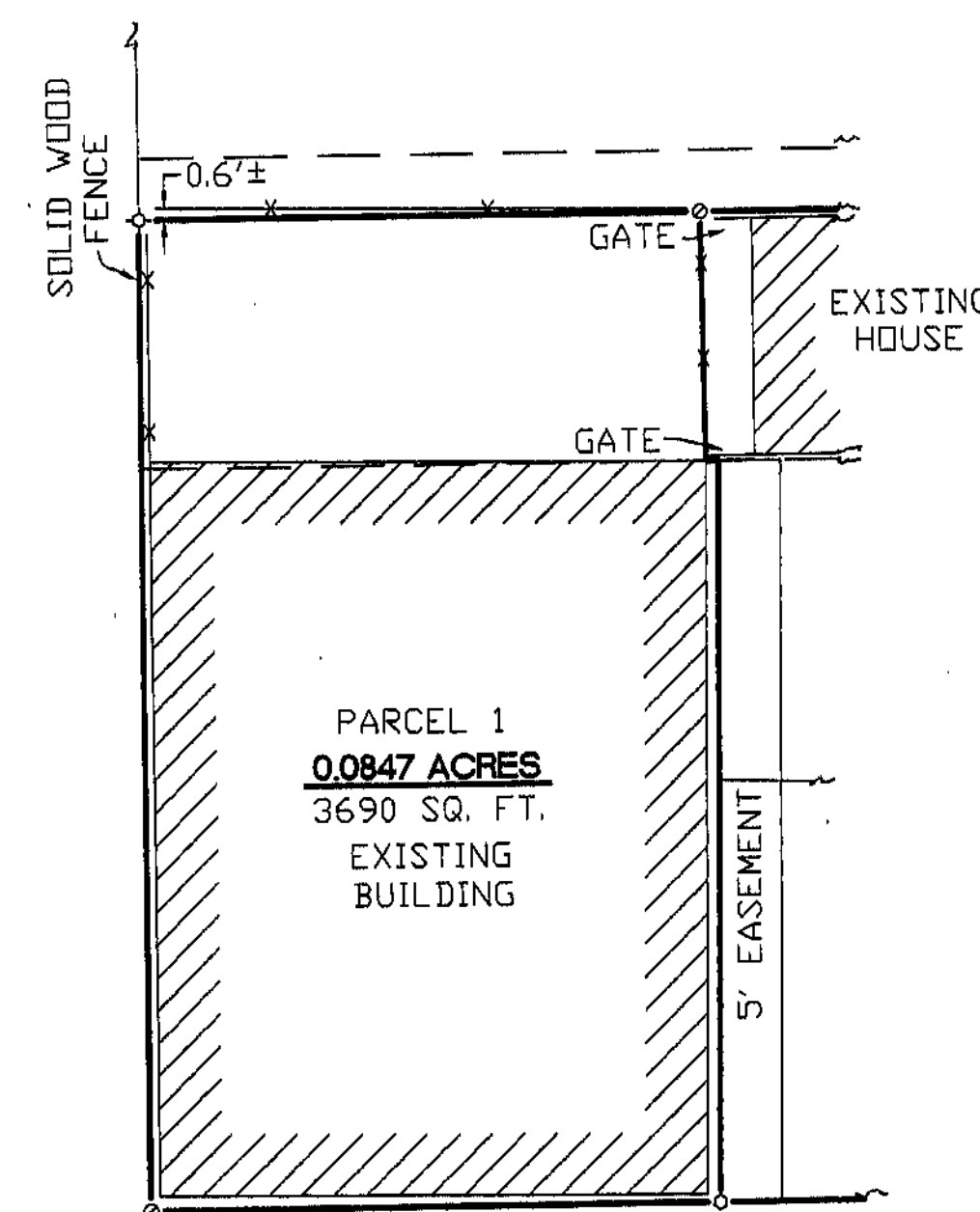
FENCE ENCROACHMENT DETAIL NOT TO SCALE
